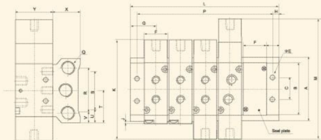
Manifold for 4A series
