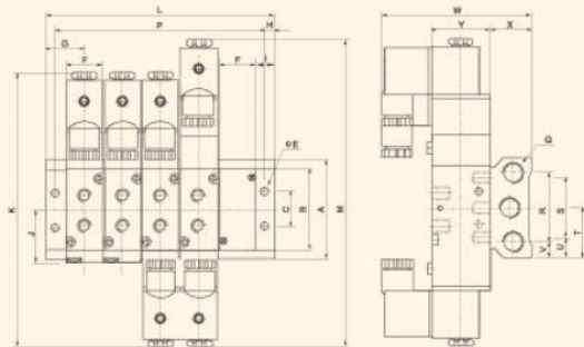
Manifold for 4V series
